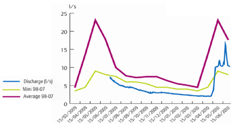
FIGURE 12: Discharge of the “Macôt-la-Plagne” spring (2009-2010). Blue: discharge 2009-2010, which was lower than the calculated average in the period 1998-2007 (purple line) and lower than the measured minima over the same period (green line).
