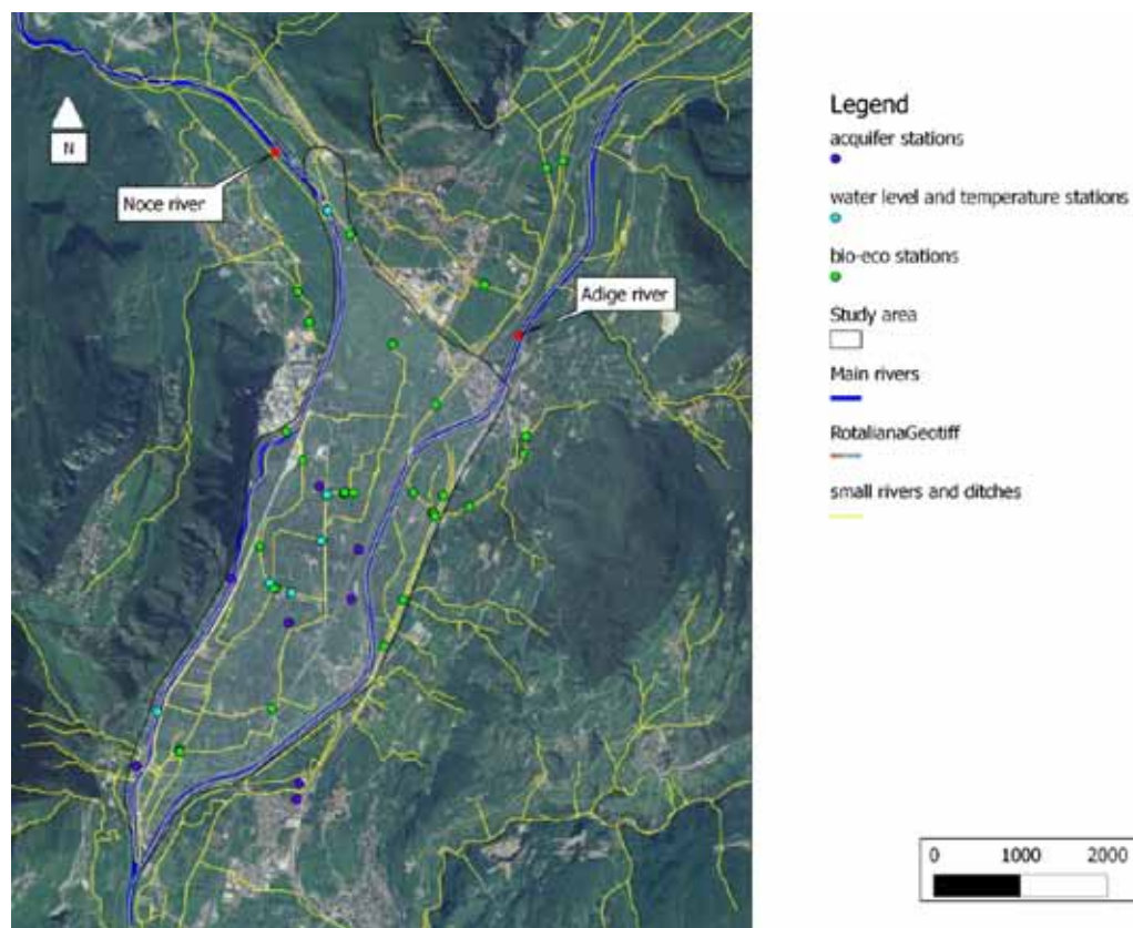
FIGURE 24: Rotaliana floodplain measuring network.
